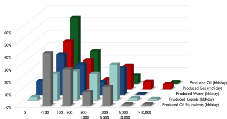
Figure 15: Failures Grouped by Well Fluid Rate Ranges, 2021
