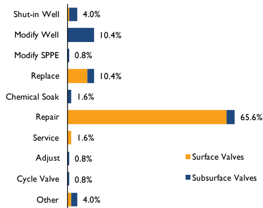
Figure 24: Reported Corrective Actions, 2021
