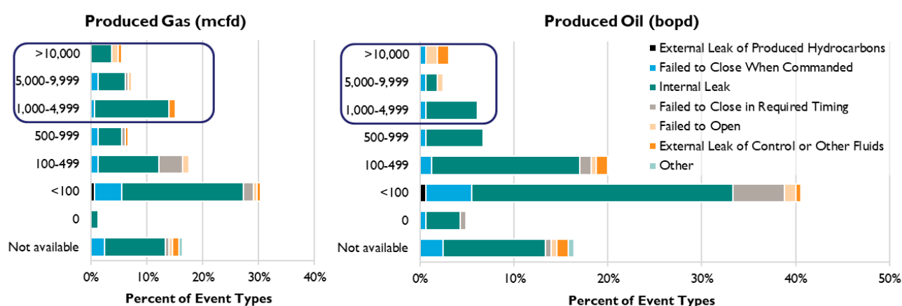
Figure 14: Type of Reported Failures by Well Rate, 2021
