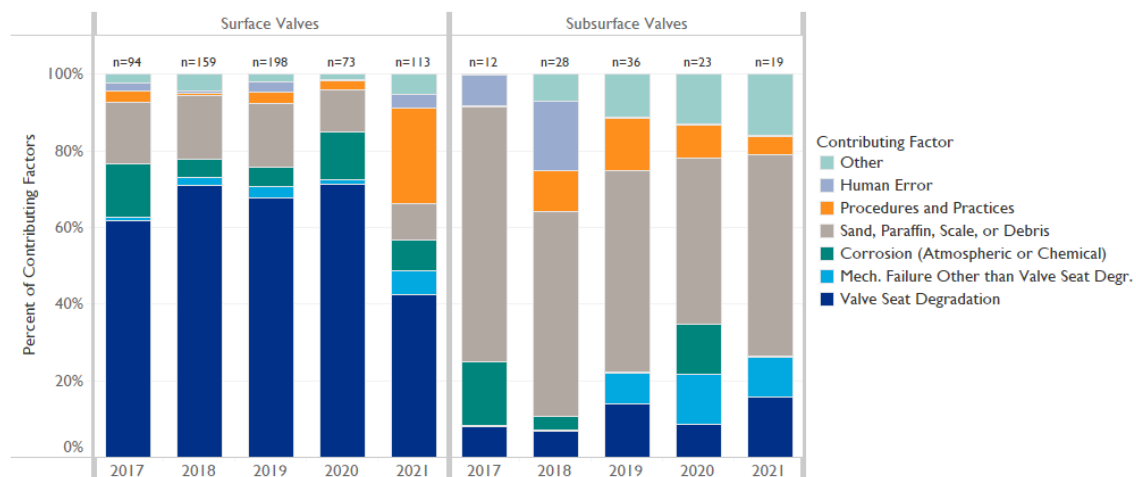
Figure 29: Factors Contributing to Equipment Failures, 2017-2021
