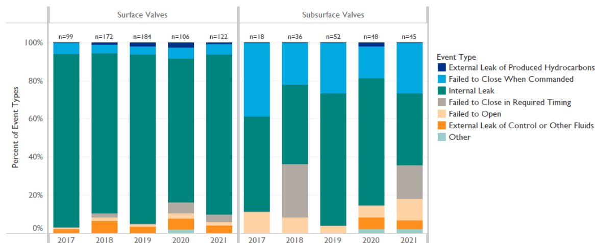
Figure 10: Failure Events by Type, 2017-2021
