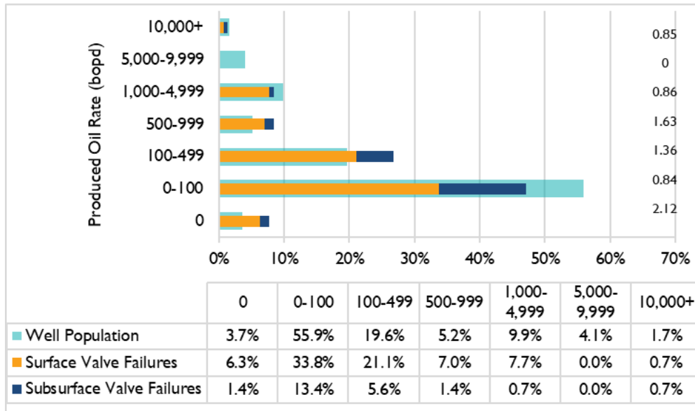
Figure 18: SPPE Failures and Active Wells by Oil Rate Group, 2021
