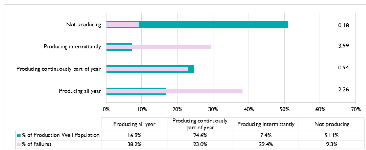
Figure 11: Production Time Group of All Production Wells vs. Wells with SPPE Failure, 2021
