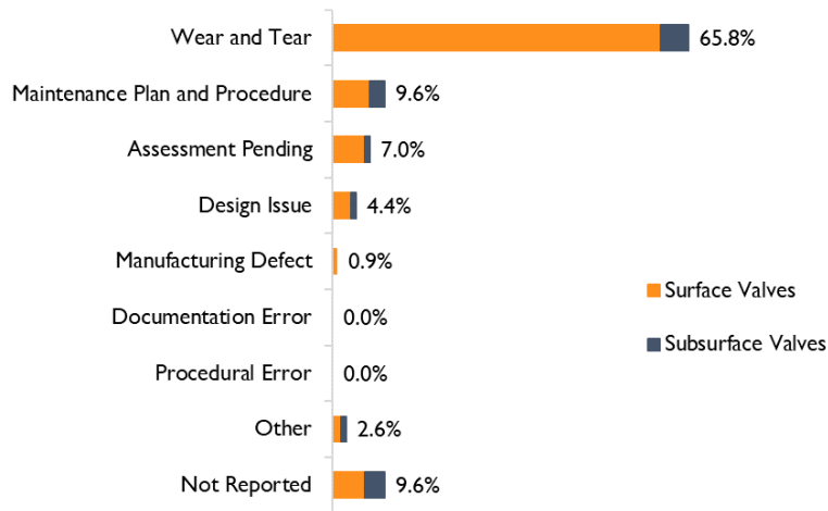
Figure 27: Root Causes of Reported Failure Events, 2021
