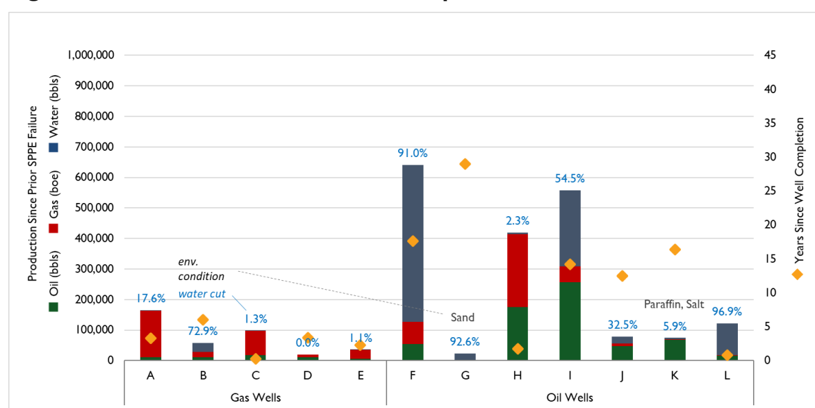
Figure 34: Production from Wells with Repeated Failures, 2021
