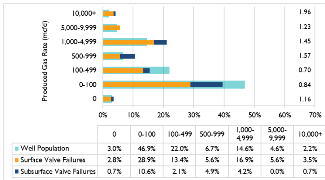
Figure 17: SPPE Failures and Active Wells by Gas Rate Group, 2021
