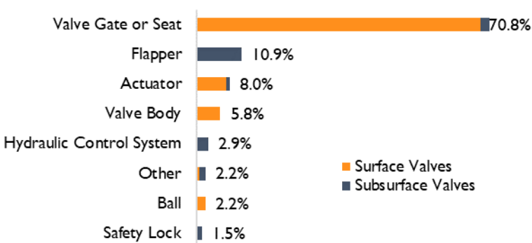
Figure 8: Failed Components in SPPE Valves, 2021
