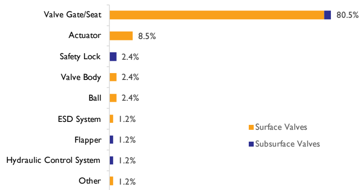
Figure 25: SPPE Components Repaired, 2021
