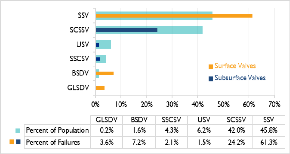
Figure 6: Reported SPPE Events by Valve Type, 2021
