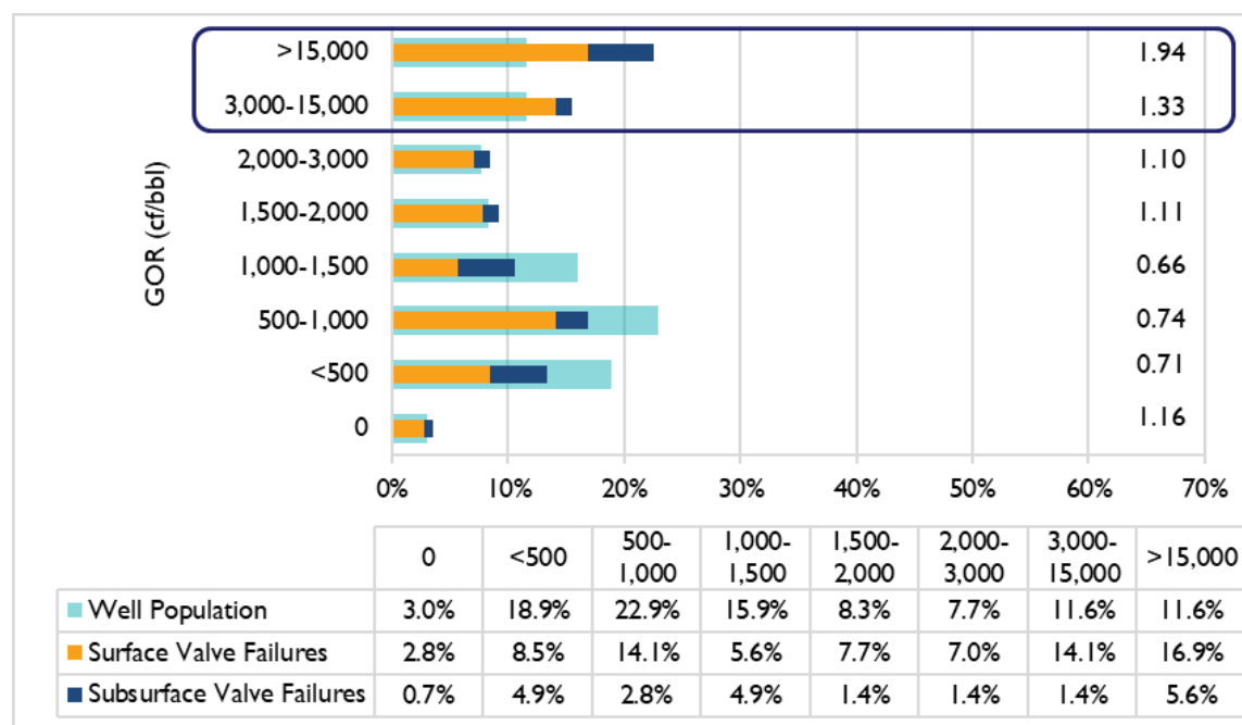
Figure 16: SPPE Failures and Producing Wells by GOR Range, 2021
