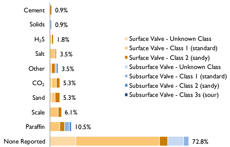
Figure 30: Well Stream Contaminants, 2021
