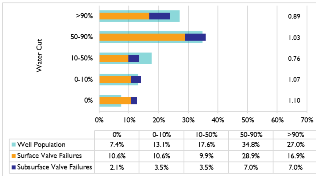
Figure 20: SPPE Failures and Active Wells by Water Cut Range, 2021
