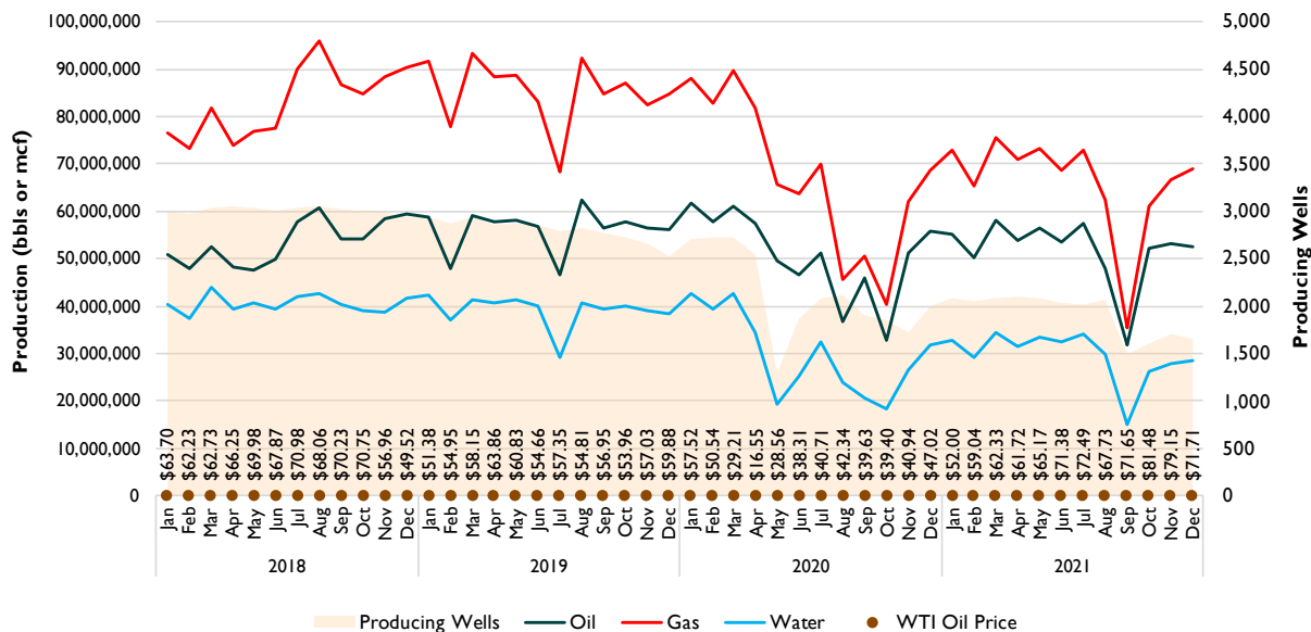
Figure 2: GOM Production, 2018-2021
