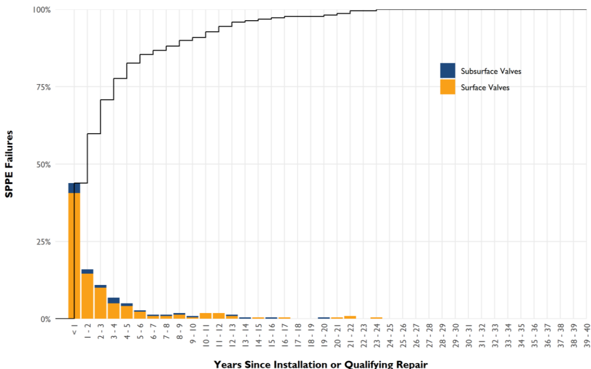
Figure 31: Time to Failure, 2017-2021
