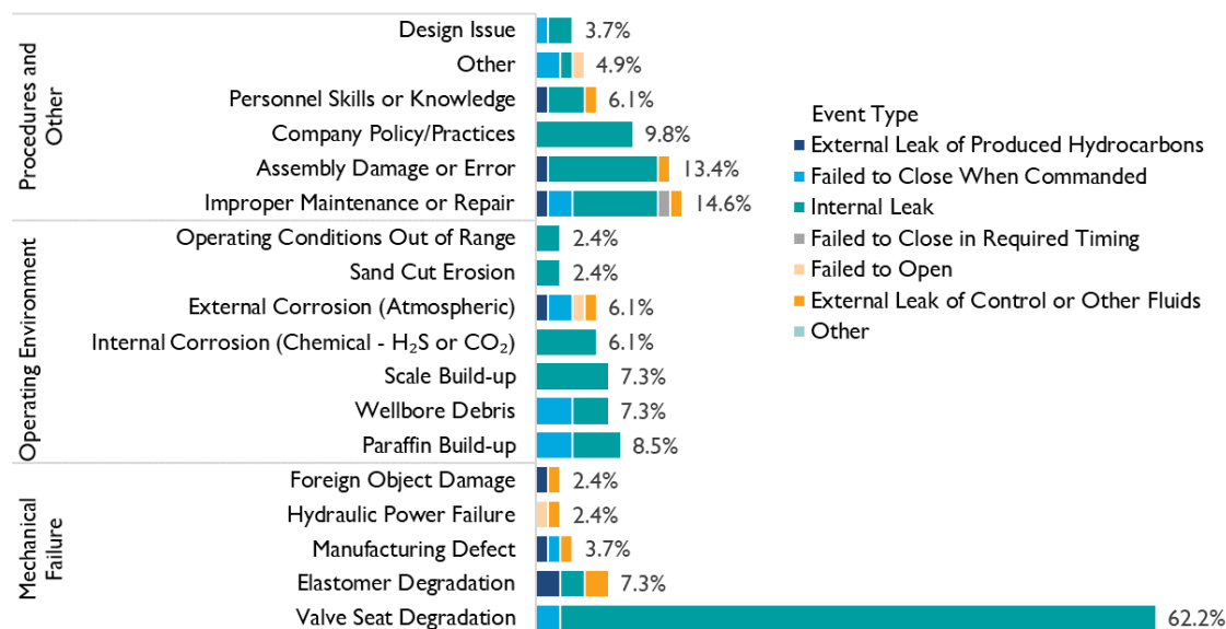
Figure 28: Factors Contributing to Equipment Failures, 2021
