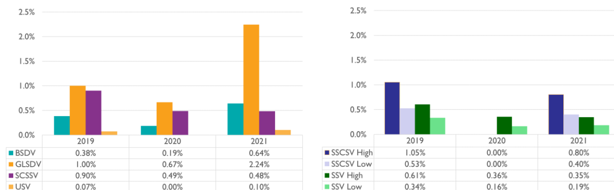
Figure 7: SPPE Failure Rates in the Gulf of Mexico, 2019-2021
