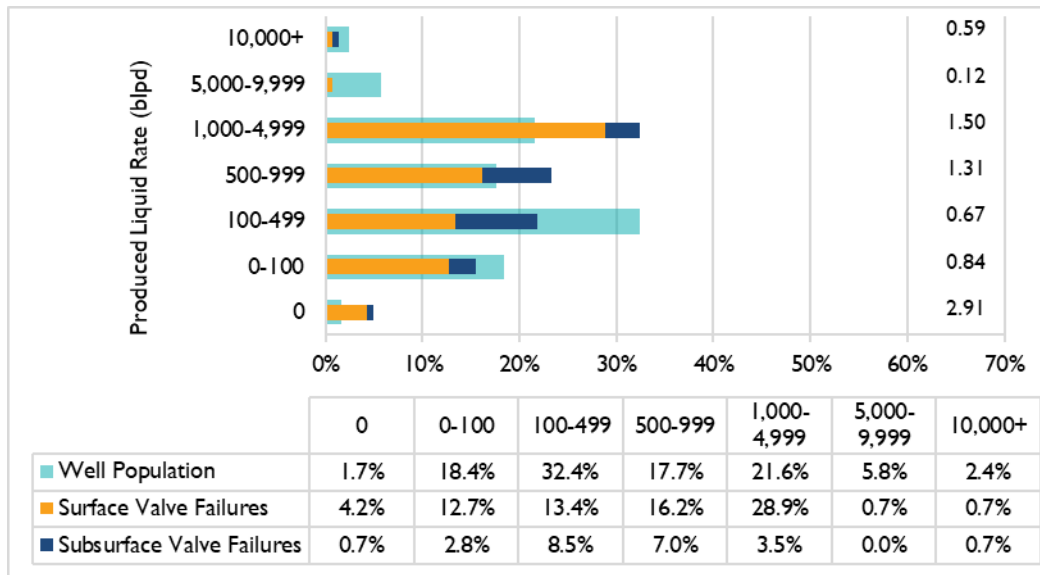
Figure 21: SPPE Failures and Active Wells by Total Liquid Rate, 2021
