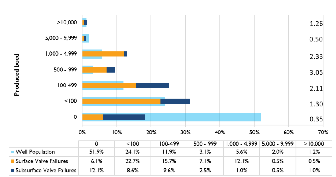
Figure 13: Well Rates for All Wells vs. Wells with SPPE Failure, 2021
