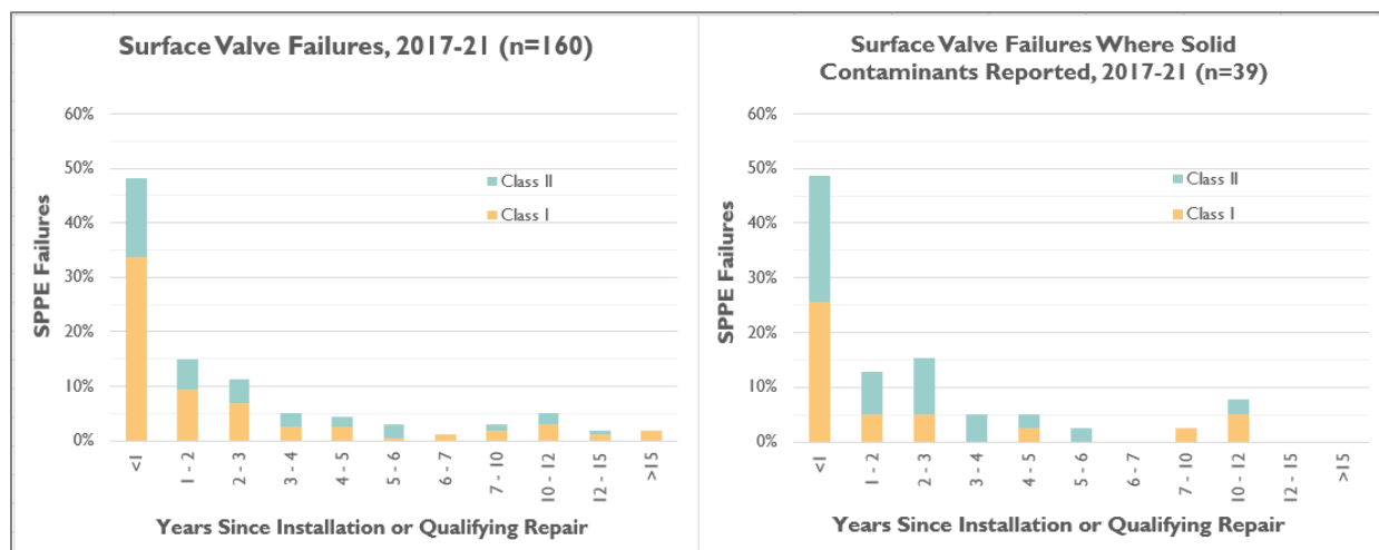
Figure 32: Time to Failure and Valve Service Class, 2017-2021
