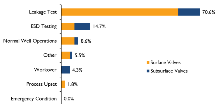
Figure 23: Failure Detection Methods, 2021
