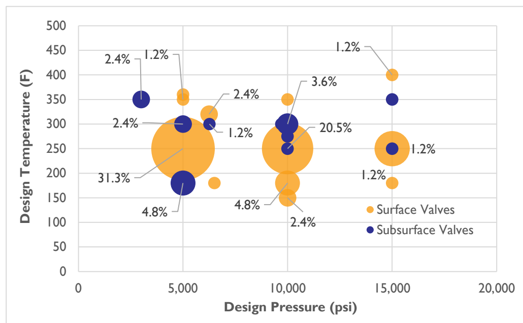
Figure 22: Percent of Failures by Valve Pressure and Temperature Ratings, 2021
