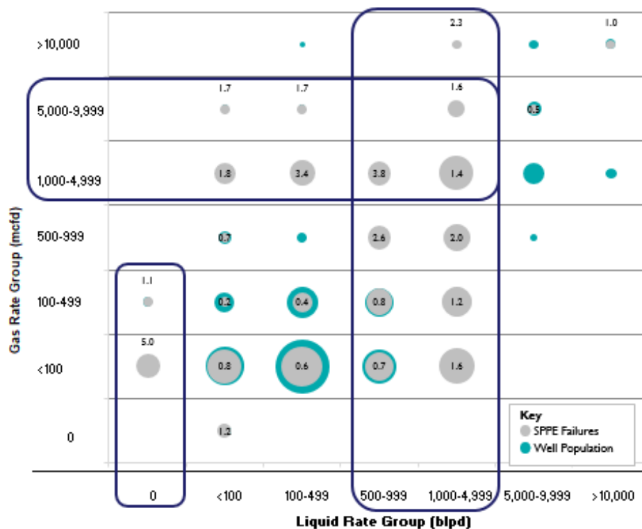
Figure 36: Gas Rate versus Liquid Rate, 2021
