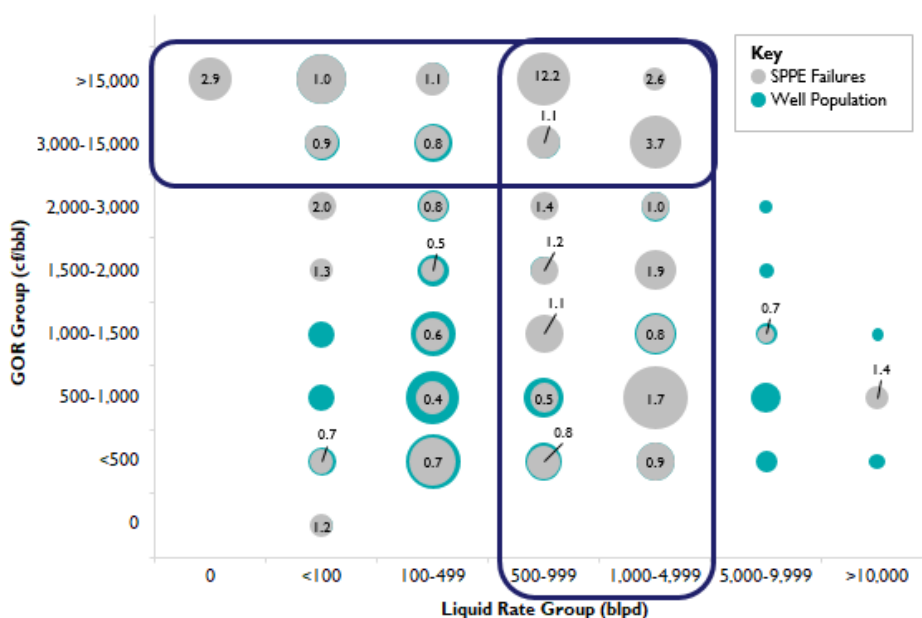
Figure 37: GOR versus Liquid Rate, 2021
