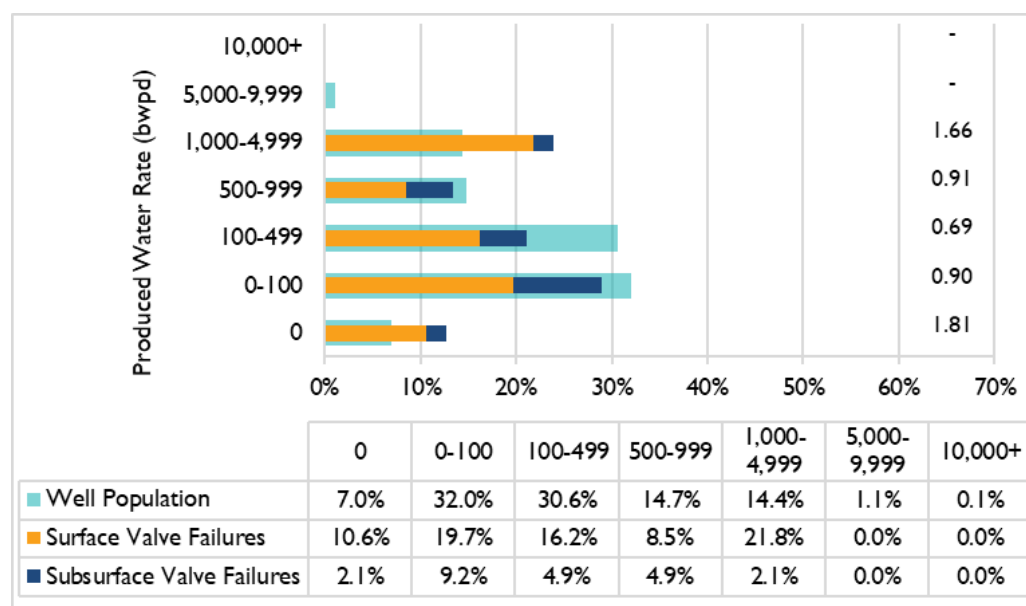
Figure 19: SPPE Failures and Active Wells by Water Rate Group, 2021
